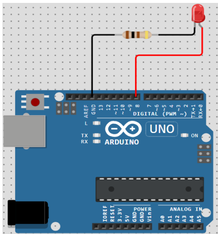
(a) LED state change without any switch
