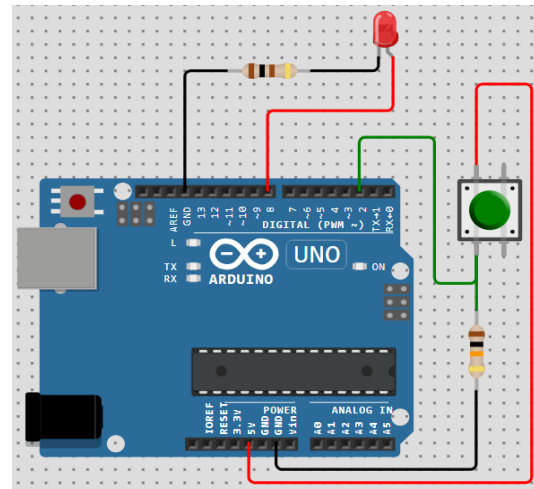
(b) LED state change with switch
