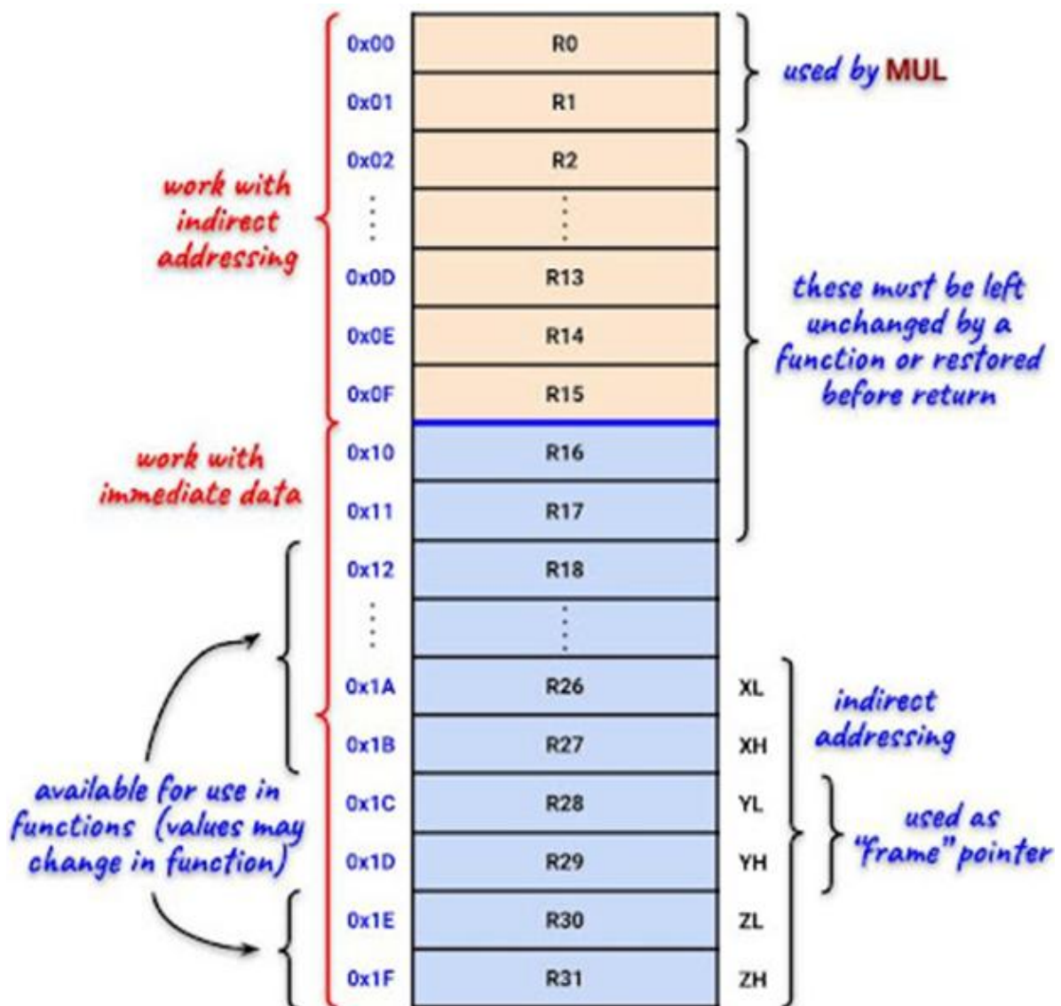
Fig. 3 General-purpose registers of the Arduino (ATMega328P)
